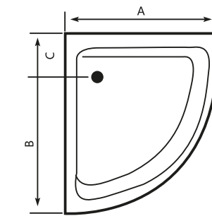
ST-101 Acrylic Shower tray
