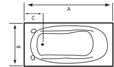
ALCO Acrylic Bathtub
